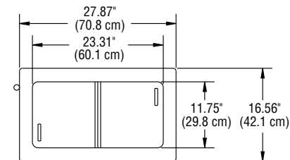
Plan View N225 & 225L
