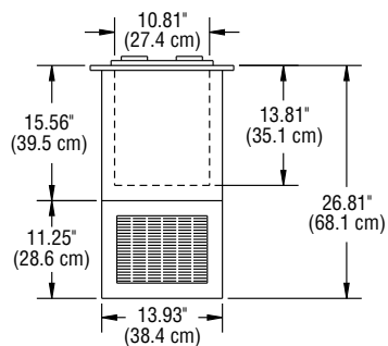
End View N225 & 225L
