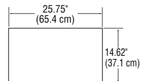
N225 & 225L Cutout Dimensions
